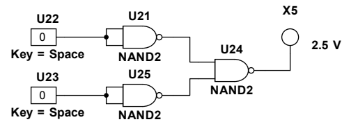
NAND AS OR
