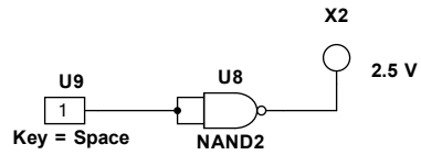
NAND AS NOT
