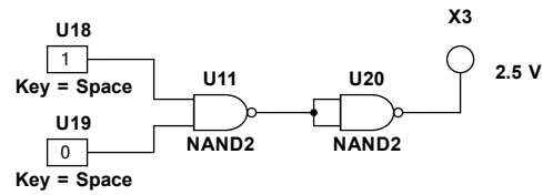
NAND AS AND
