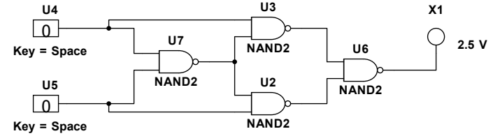
NAND AS XOR
