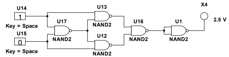
NAND AS XNOR
